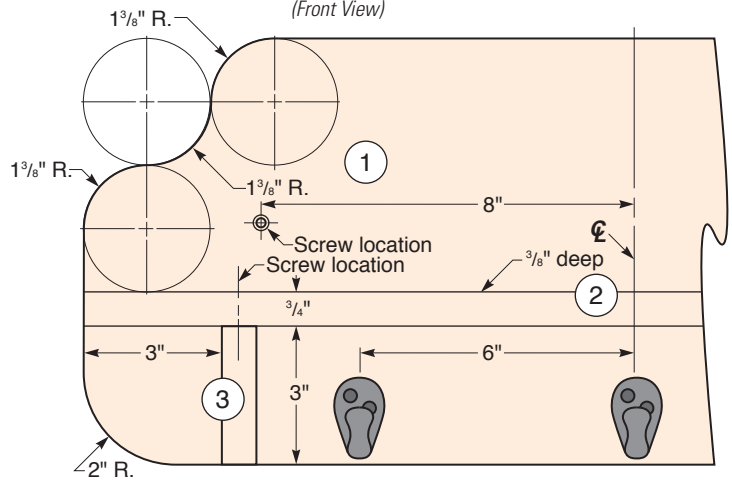
Shelf (Front View)
